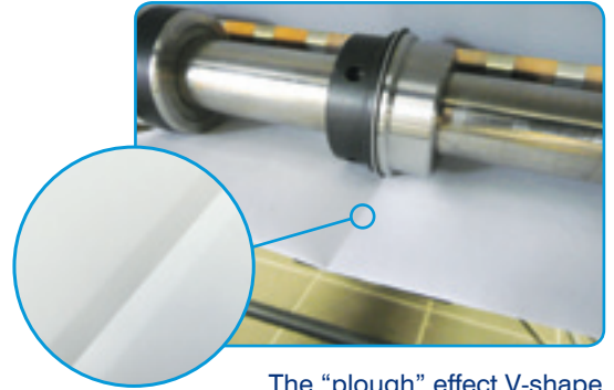
The “plough” effect V-shape score created by steel scoring devices
