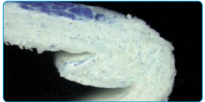
The reverse crease method gets to work on the outside of the fold, pushing the fibres inward
